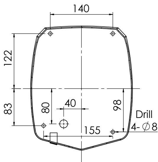
INSTALLATION TEMPLATE
