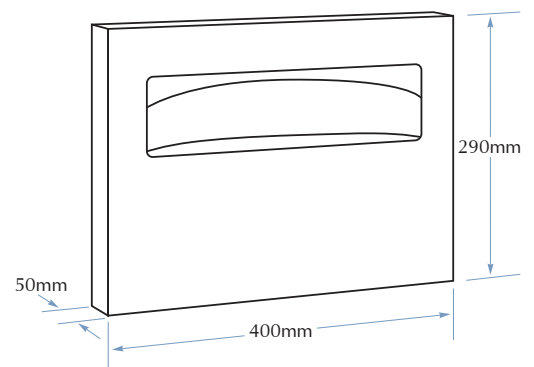
583 Surface Mounted
