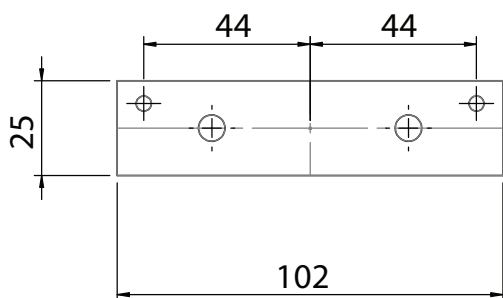
Anchor Plate ((optional))
